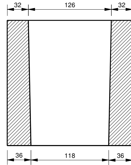
END X-SECTION
