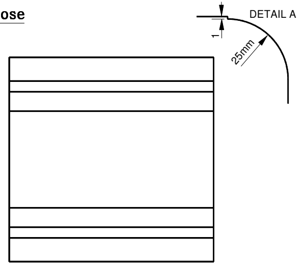
END VIEW
