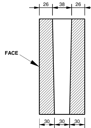
END X-SECTION
